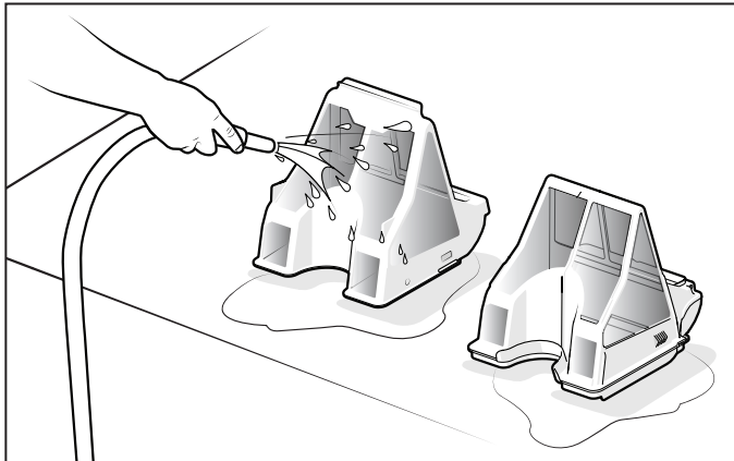
Figure 23. Remove and Wash the Filter Canisters
