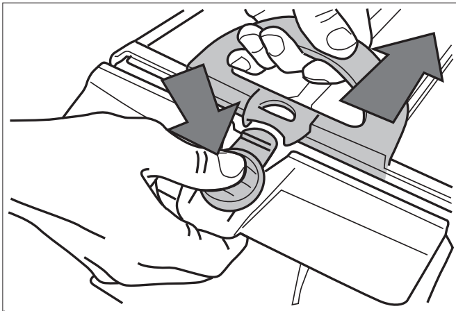
Figure 20. Open Filter Canister Assembly
